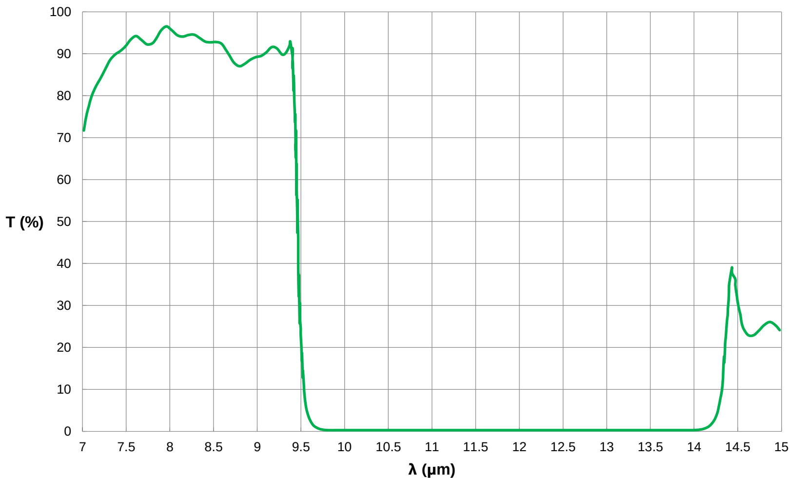
9.5 \mu m Shortpass Filter: OD \geq 3.0 Coating Performance FOR REFERENCE ONLY
