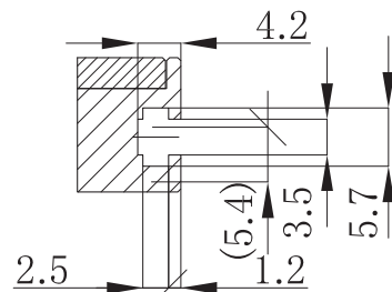
M3 Nut slot Detail drawing
